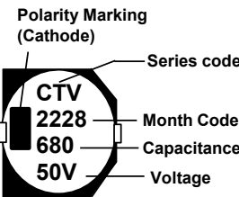
Fig.2 ΦD≥12.5mm
