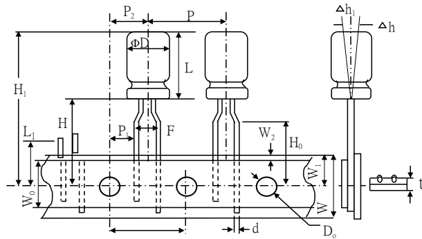
Fig.3( \Phi 5-\Phi 8 )
