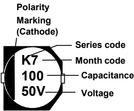
Fig.1 ΦD=4~ 10mm
