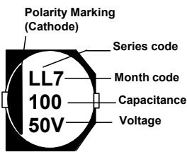
Fig.1 ΦD=5~ 10mm
