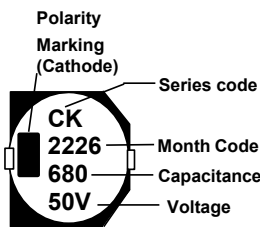
Fig.2 ΦD≥12.5mm
